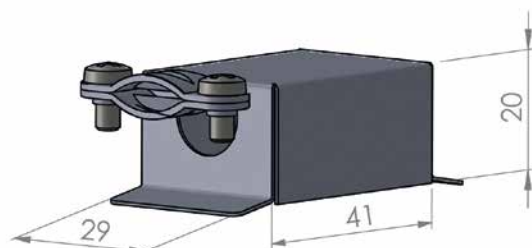
CT-15 TANGENTIAL Anschlussbox / Connection box
